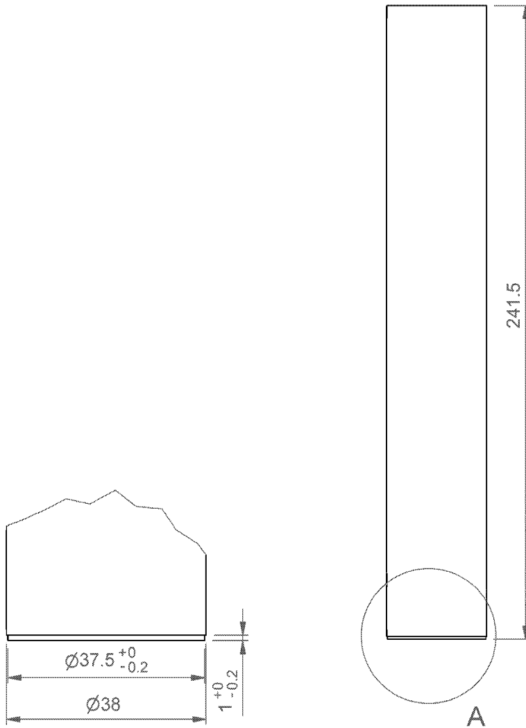
DETAIL A
